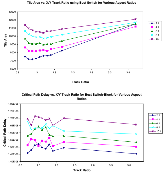
Figure 9: Plot of tile area and critical path delay versus track ratio for each aspect ratio. The ideal switch block is used for each data points.
