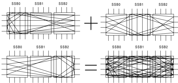
Figure 3: The tracks of a rectangular switch block are the summation of tracks from three individual Imran Patterns.
